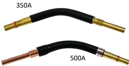
NO.6 SWAN NECK
