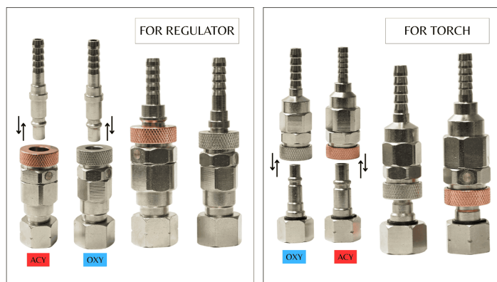
WELDING COUPLING
