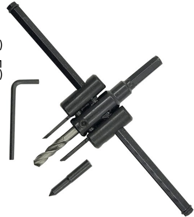
ADJ.HOLE CUTTER
