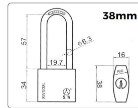
PAD LOCK [ANTI-CUT]
