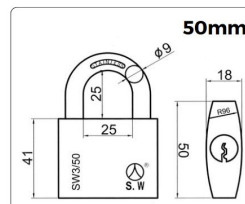
STAINLESS STEEL PAD LOCK—SHORT
