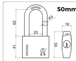
STAINLESS STEEL PAD LOCK—LONG
