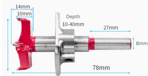
FORSTNER BIT WITH STOPPER
