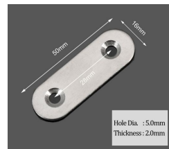
STRAIGHT BRACKET
