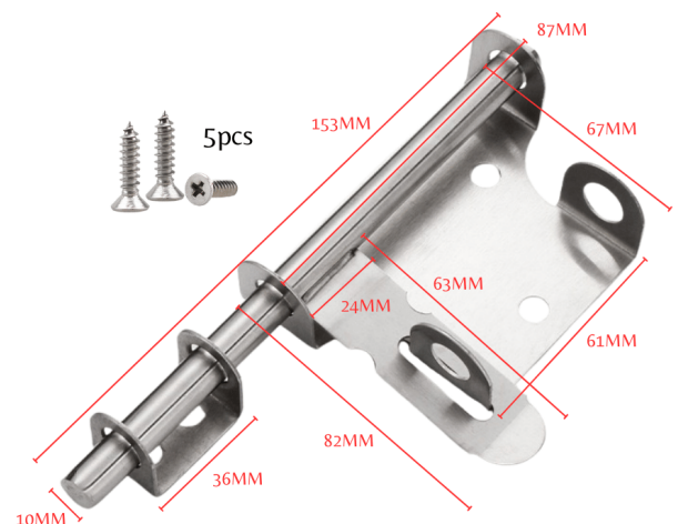
BARREL BOLT—6"/ 2 EAR | S.STEEL [4-057]
