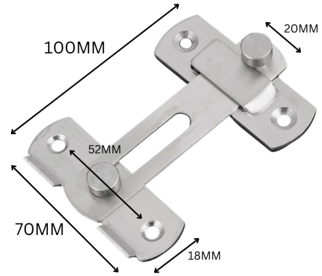
SLIDING DOOR LATCH—4" (L70MM x W100MM)
