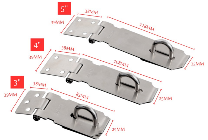
HASP & STAPLE - 304 S.STEEL/H.DUTY
