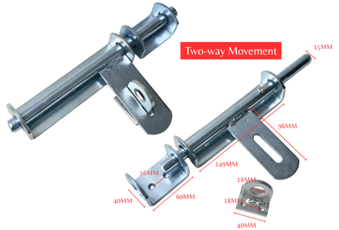
BARREL BOLT -9" (GALVANIZED)
