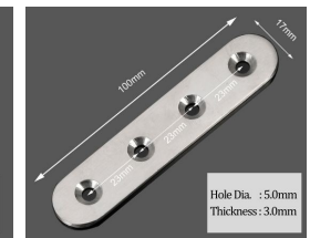
STRAIGHT BRACKET
