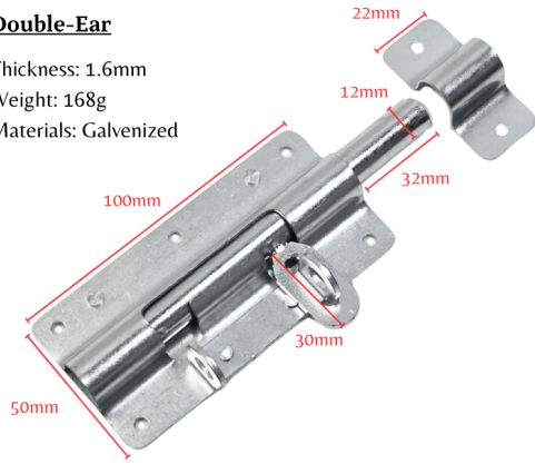
BARREL BOLT -5" / DOUBLE EAR (GALVANIZED)
