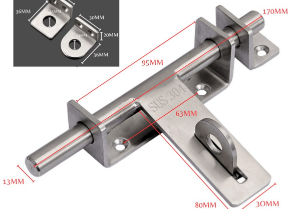
BARREL BOLT—170MM | S.STEEL [4-056]
